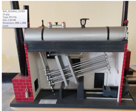
A . Babcock and Wilcox Boiler
